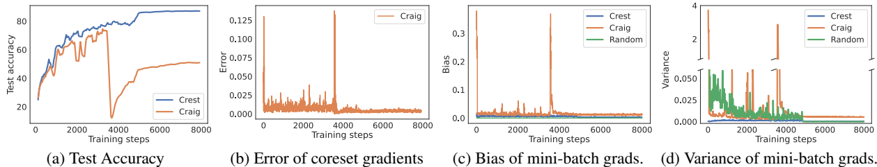
Figure 1: Training ResNet20 on CIFAR-10. (a) 10% CRAIG coresets selected at the beginning of every epoch from full data may perform very poorly. This is because, (C1): (b) Coresets may have a large error: \|\mathbf{g}_{t,S} - \nabla \mathcal{L}(\mathbf{w}_t)\| , after a few training iterations; and (C2): Gradient of weighted mini-batches selected from the coresets may have a (c) large bias \|\mathbb{E}_i[\mathbf{g}_{t,\mathcal{M}_i}] - \nabla \mathcal{L}(\mathbf{w}_t)\| and (d) large variance \mathbb{E}_i[\|\mathbf{g}_{t,\mathcal{M}_i} - \nabla \mathcal{L}(\mathbf{w}_t)\|^2] , where \mathcal{M}_i \in S is a mini-batch and \mathbf{g}_{t,\mathcal{M}_i} = \mathbb{E}_{j \in \mathcal{M}_i}[\gamma_j \mathbf{g}_{t,j}] . In contrast, our CREST coresets are nearly unbiased, and have a smaller variance than random mini-batches of same size.
