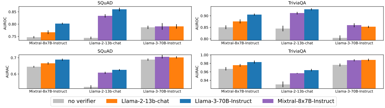
Figure 3: Comparison between approximated ceiling performances using only P^{\text{self}} (gray) and those using both P^{\text{self}} and P^{\text{cross}} . The x-axis shows the target model, and the colors indicate the verifier model, as shown in the legend. We observe a clear improvement when a verifier model is used.
