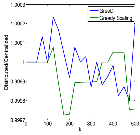
(b) Kosarak
