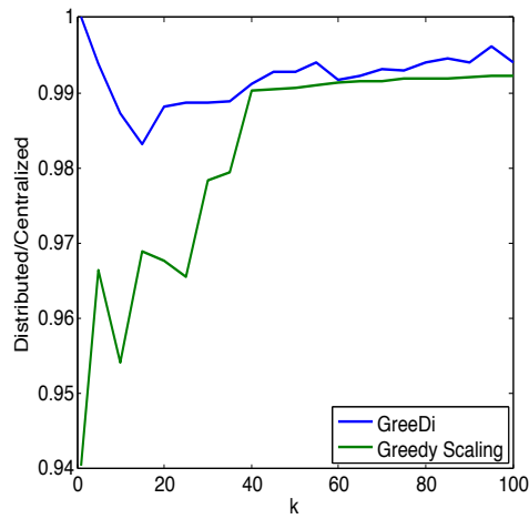
(a) Accidents
